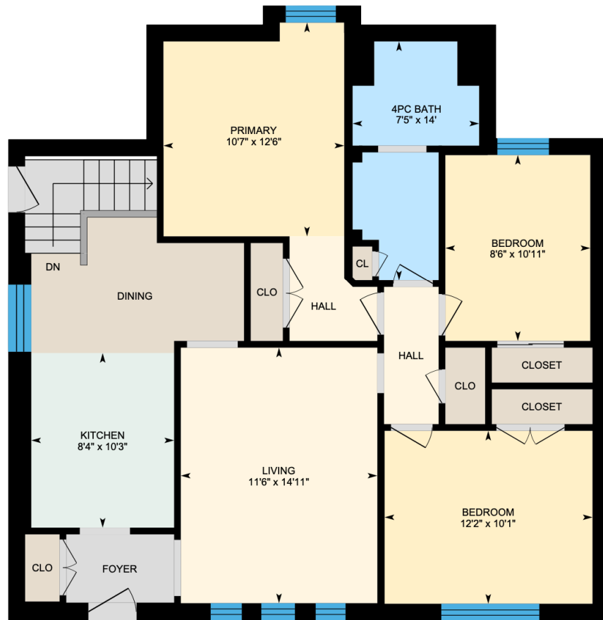
First Floor Plan Total Sqft: 1109.00
