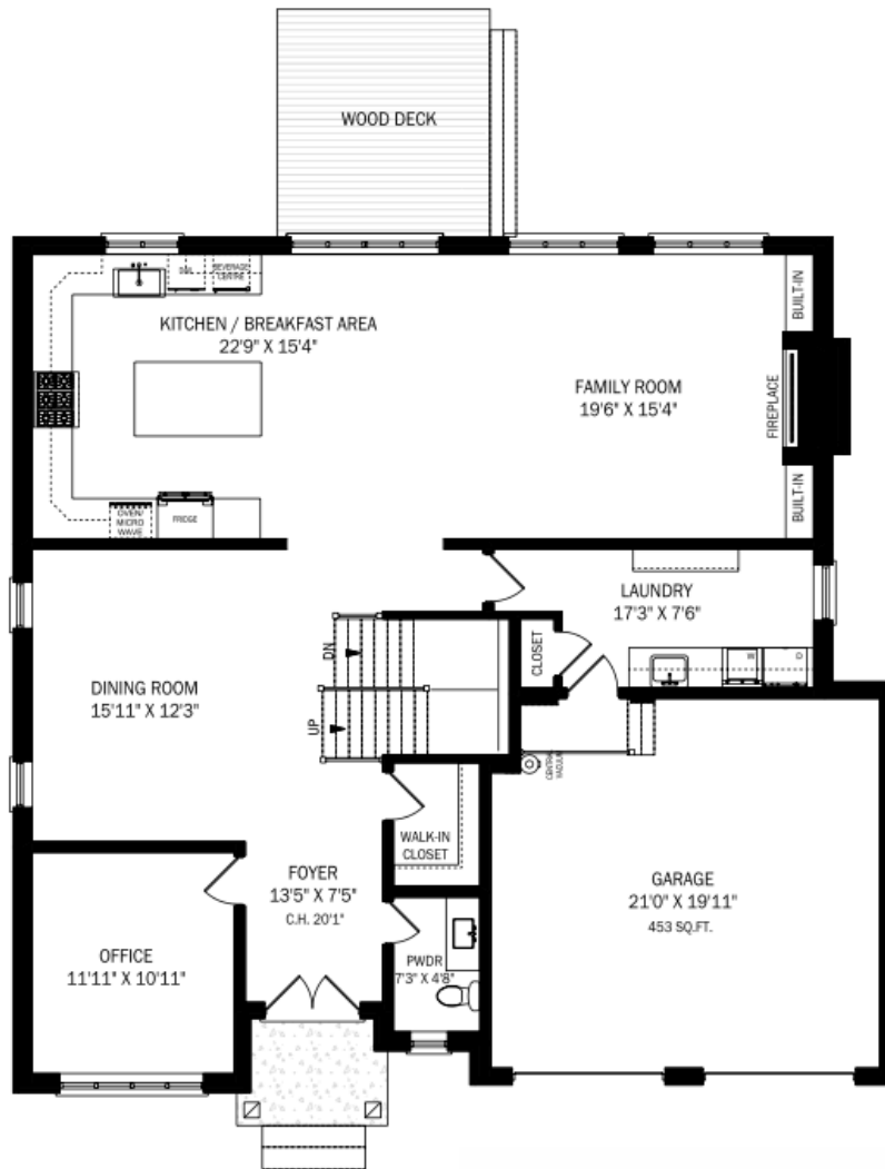
Main Floor - 1616 SQFT Ceiling Height 10'
