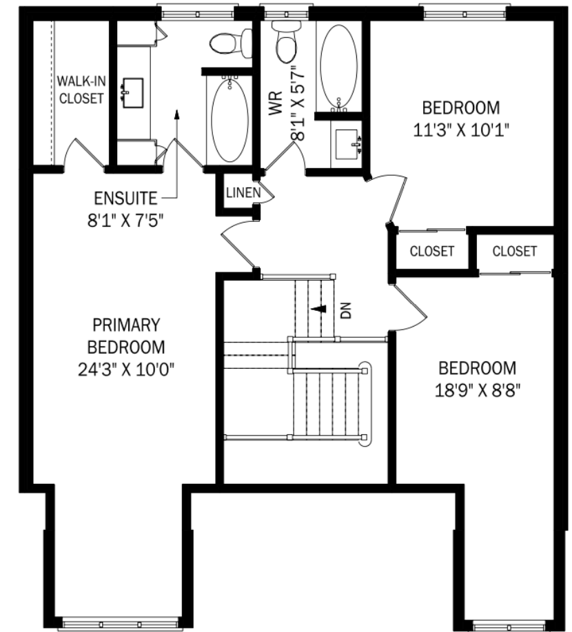
Second Floor - 902 SQFT Ceiling Height 8'
