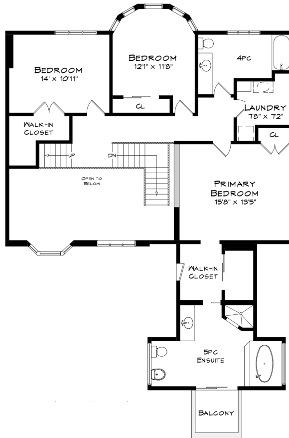
Second Floor - 1281 SQFT + 254 SQFT Open to Below
