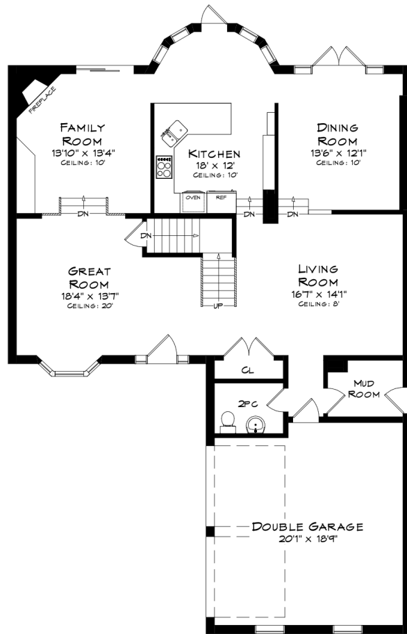
Main Floor - 1362 SQFT + 415 SQFT Garage
