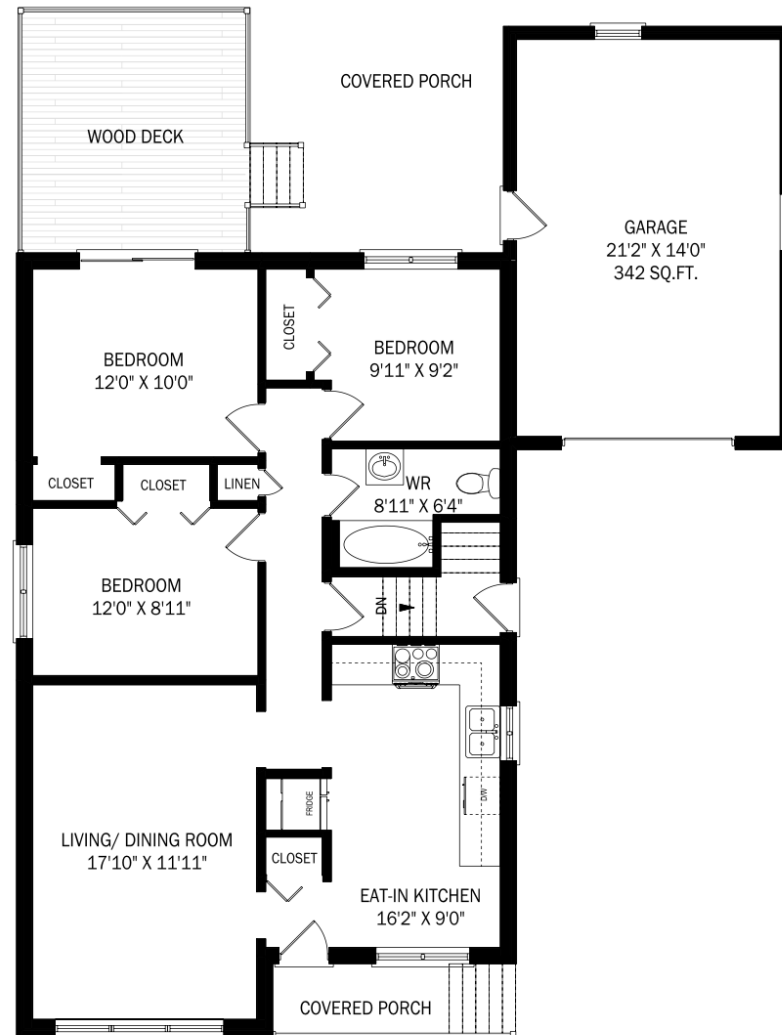
Main Floor - 1064 SQFT
