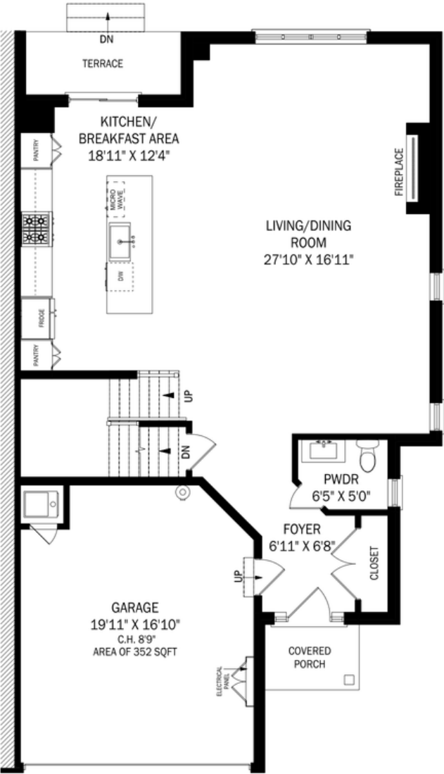
Main Floor - 1039 SQFT - 9' Ceilings
