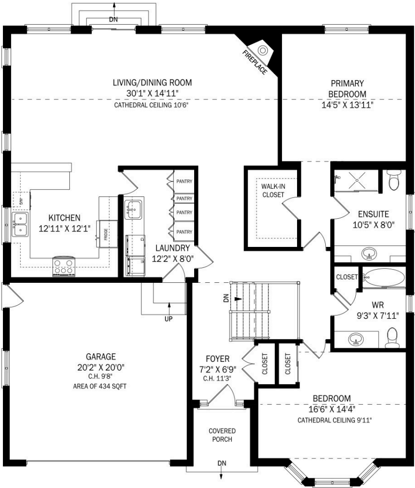
Main Floor - 1840 SQFT
